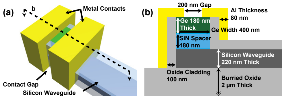
Fig. 1. (a) 3-D drawing of the proposed device showing the metal-clad box sitting on the terminated input waveguide. Splitting down the center of the waveguide shows (b) the interior components of the cavity and device can be seen.
